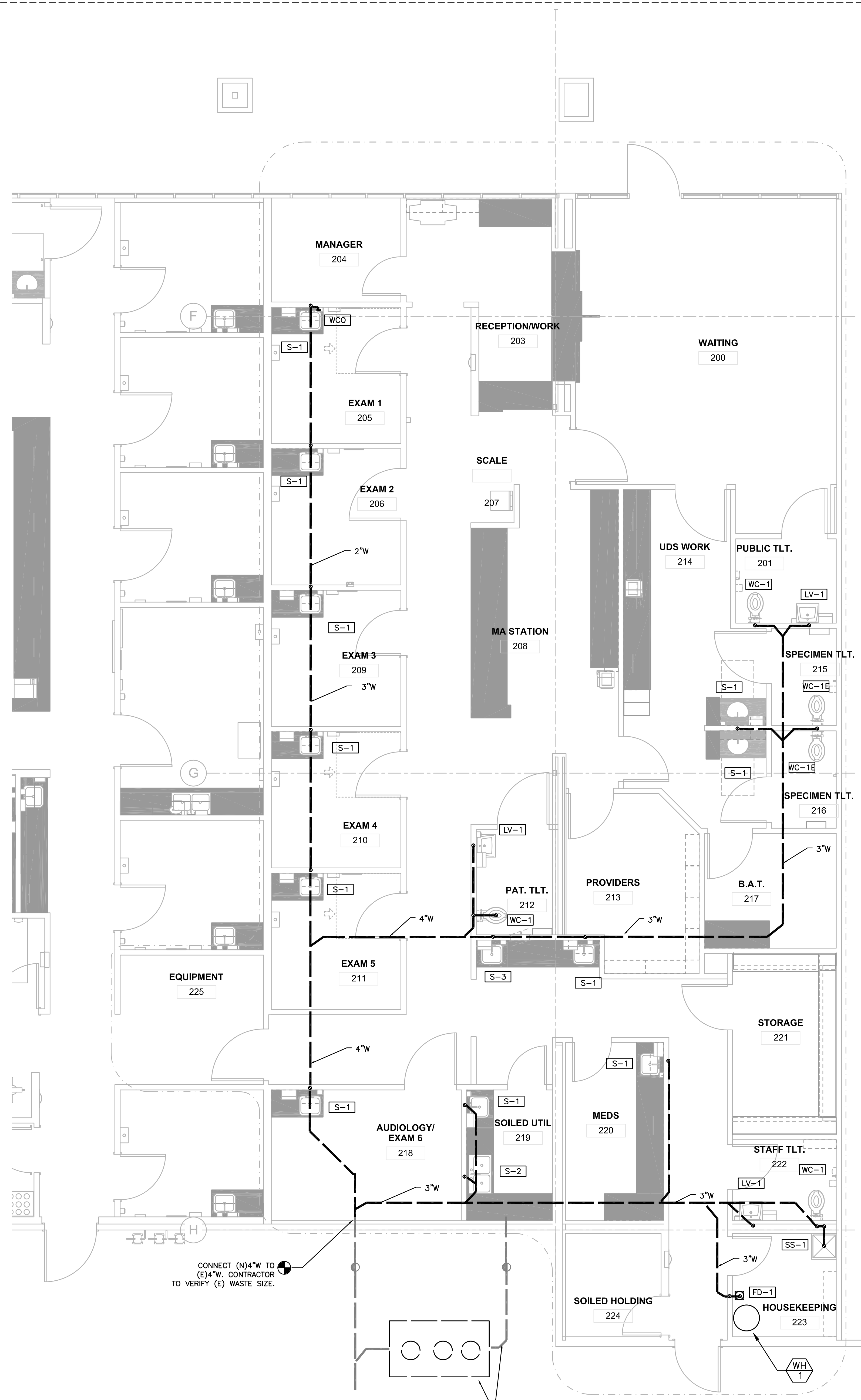
1 UNDERSLAB PLUMBING PLAN P1.1 SCALE: 1'-0" = 1/4"
